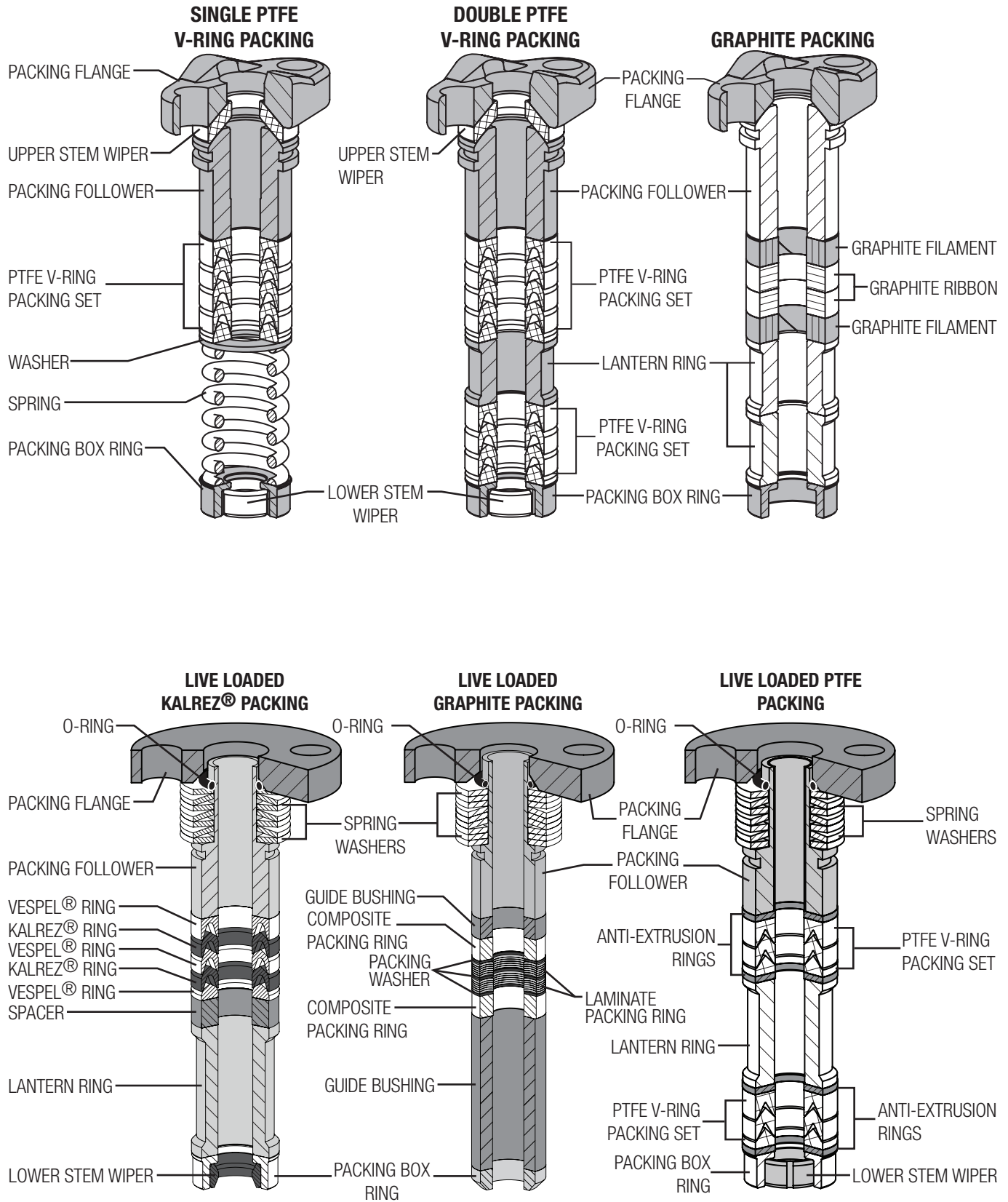
Figure 9 Typical Packing Arrangements
