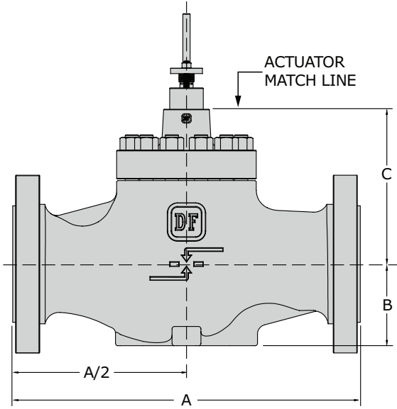
FLANGED VALVE ASSEMBLY
