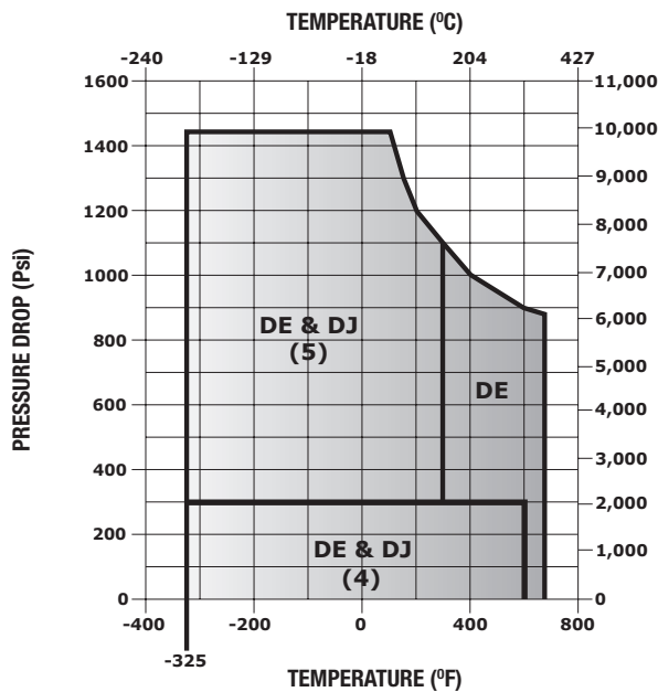
TRIM DE & DJ WITH CF8M ASME CLASS 600 VALVES
