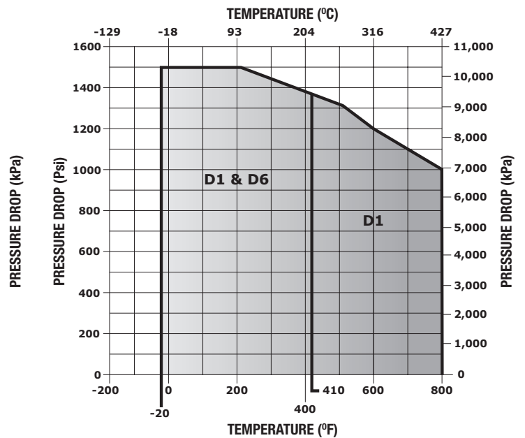
TRIM D1 & D6 WITH WC9 FOR ASME CLASS 600 VALVES
