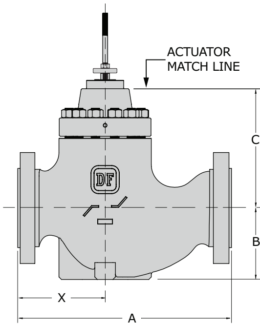
12X8" NPS (300x200 DN) FLANGED VALVE ASSEMBLY
