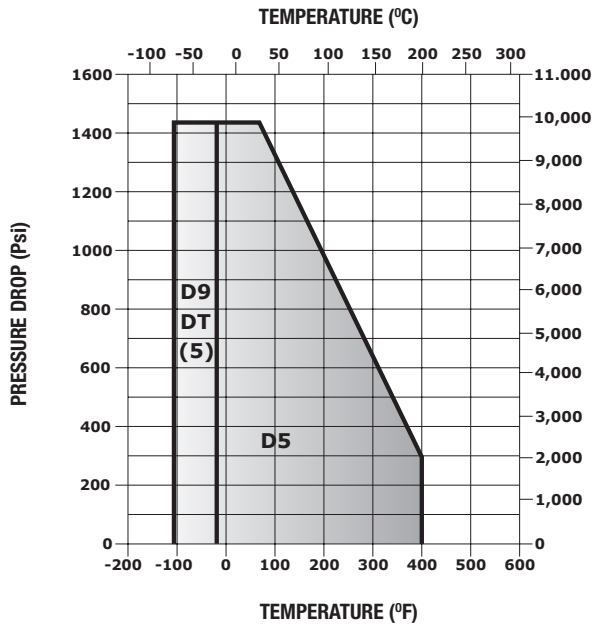
TRIM D5, D9, & DT FOR PTFE SEATED ASME CLASS 600 VALVES
