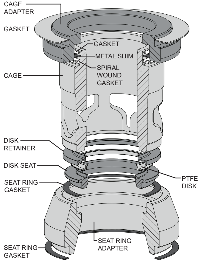
Figure 6 Reduced Trim Assembly Diagram
