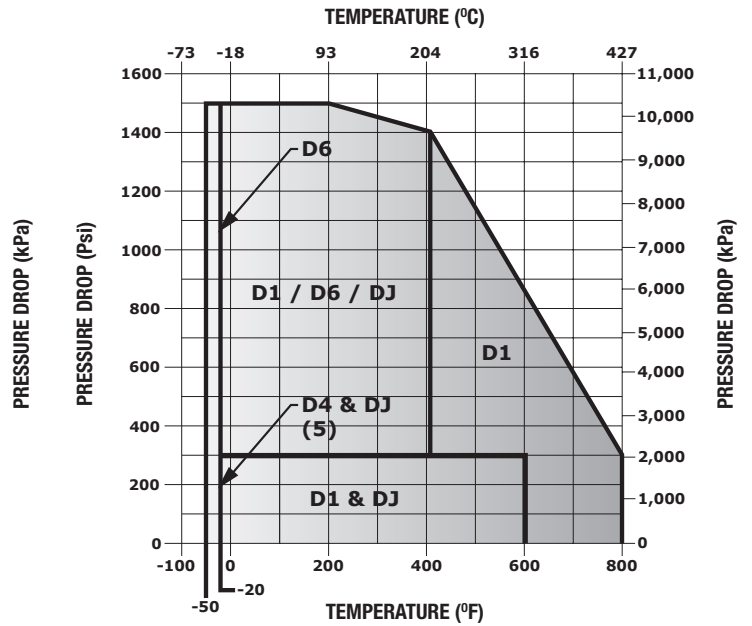
TRIM D1, D4, D6, & DJ WITH LCC OR WCC FOR ASME CLASS 600 VALVES
