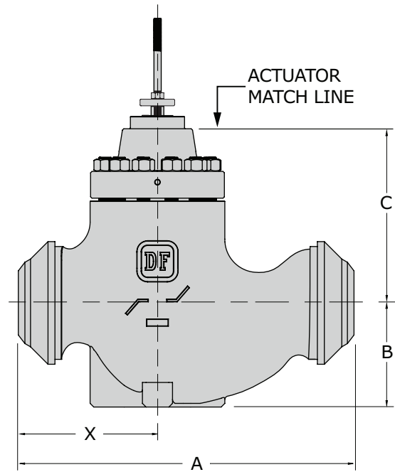
12X6" NPS (300x150 DN) BUTTWELD VALVE ASSEMBLY
