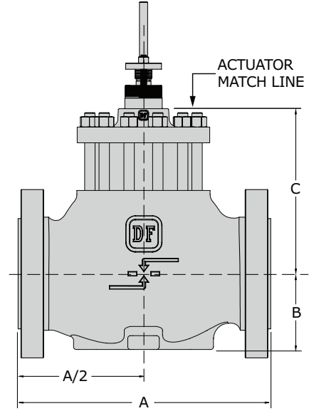
FLANGED VALVE ASSEMBLY FOR LOW-NOISE TRIM
