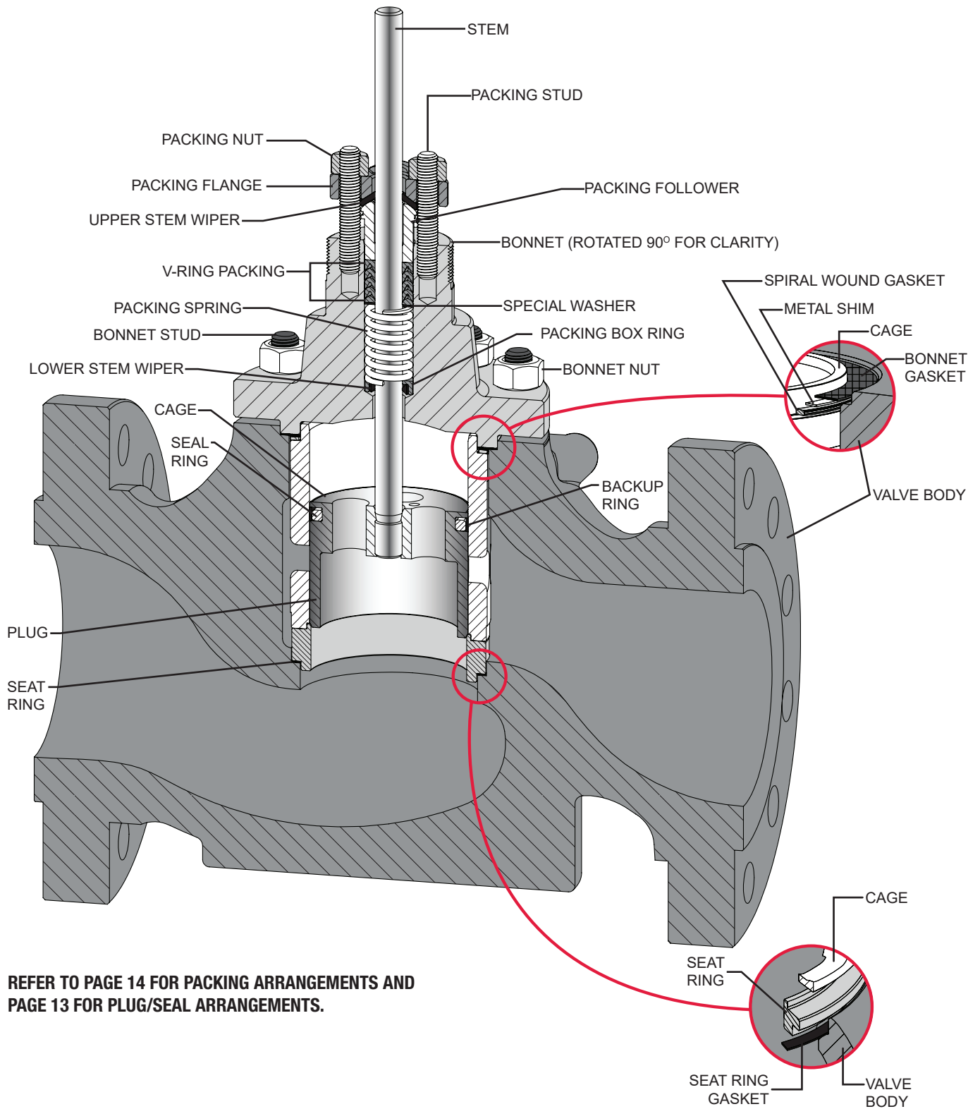
Figure 3 Standard Valve Assembly - 7 Inch (177.8mm) Port and Under
