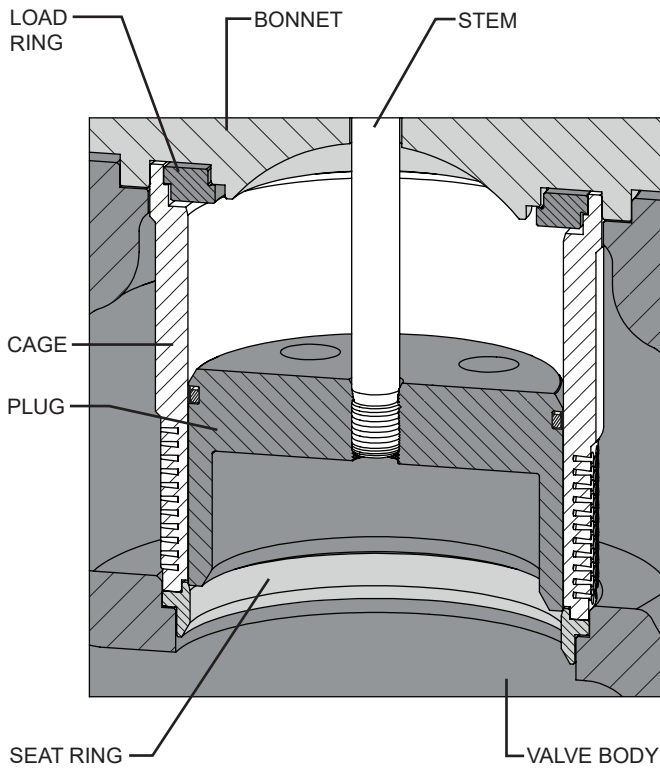
Figure 5 10x8" & 12x8" NPS (250x200 & 300x200 DN) Anti-Cavitation Valve Assembly with Load Ring
