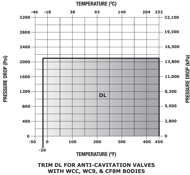
Figure 12 Typical Valve Trim Pressure and Temperature Limitations for Anti-Cavitation Trim
